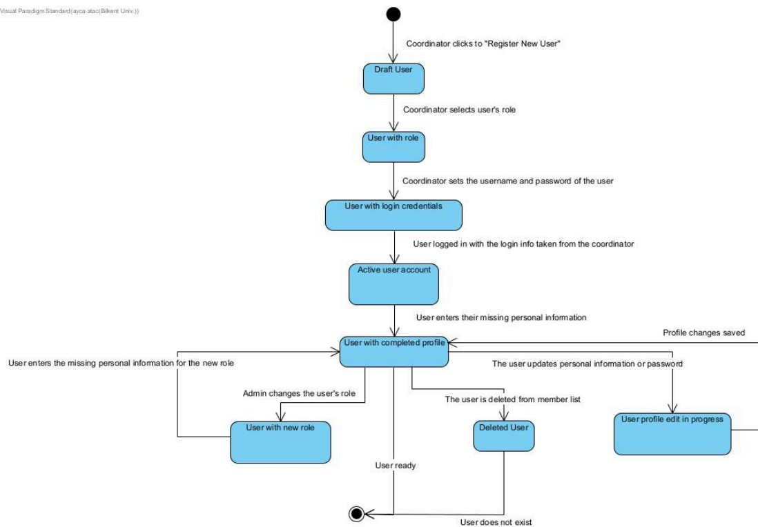
Figure 14: The state diagram of a user object
