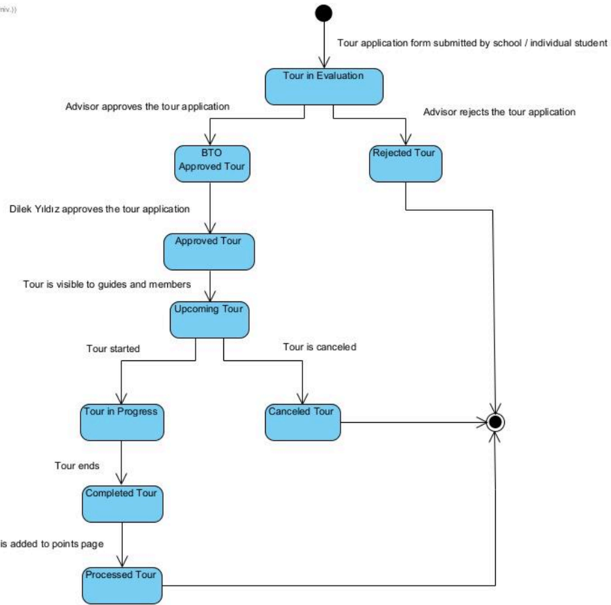
Figure 12: The state diagram of the tour object
