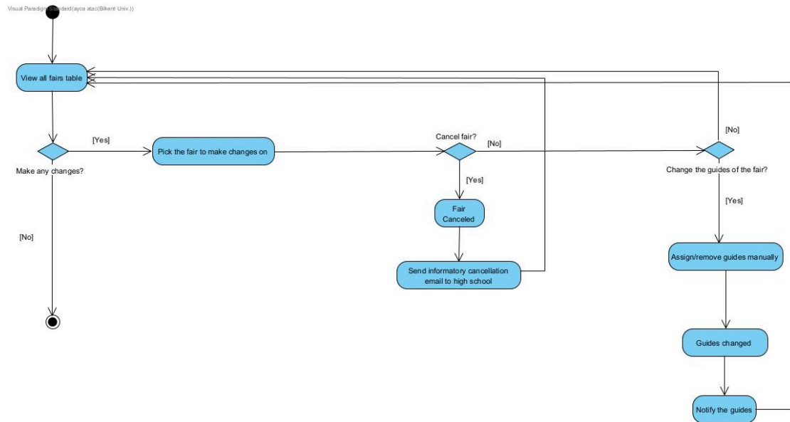
Figure 7: The cancelation and editing of already existing and approved fairs by the coordinator or director
