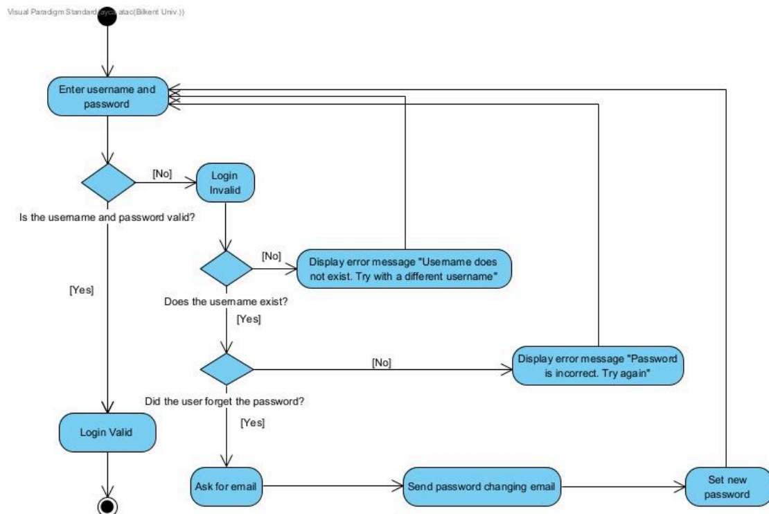
Figure 2: The login operations for members with accounts
